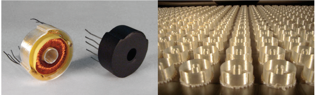
Kelly Manufacturing makes toroid housings using ULTEM 9085 on an additive manufacturing system. The method requires no tooling and offers the tight tolerance needed for this device.
